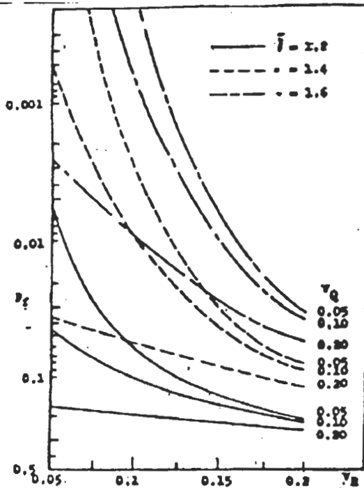
Figure 7. Probability of failure.
