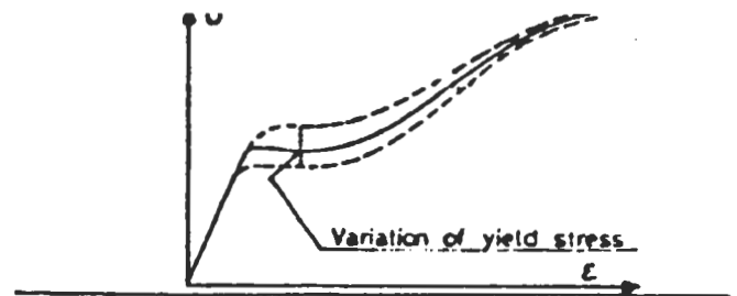
Figure 2. Stress-strain diagram.
